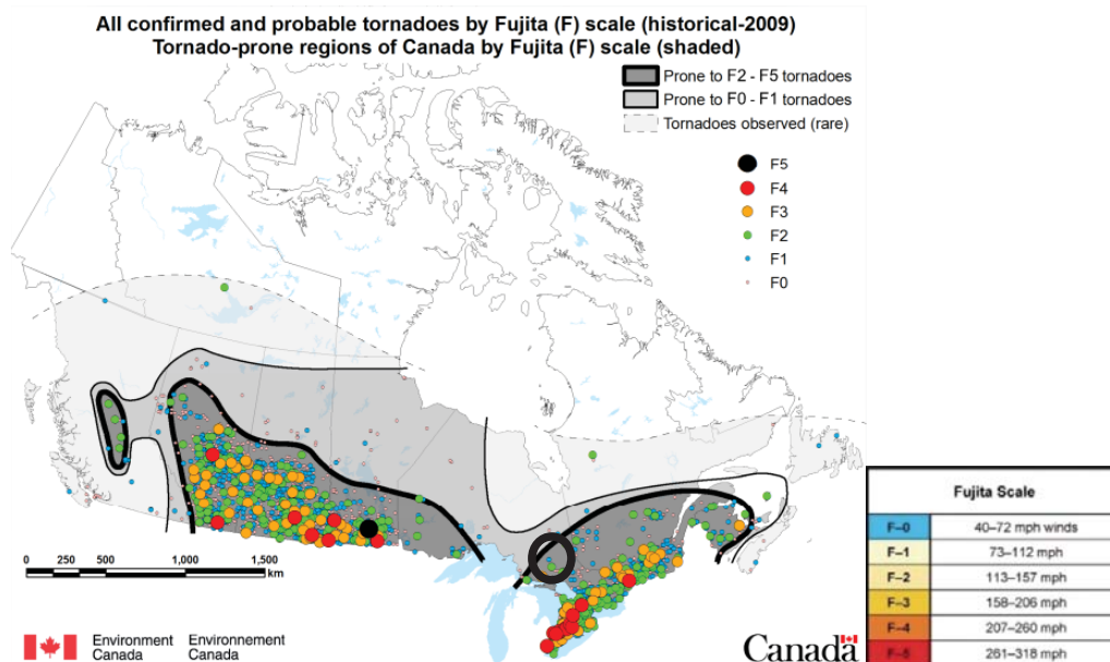
Figure 4 Map showing the F0-F1 and F2-F5 tornado prone areas as well as a 'rare occurrence' area, with all known Canadian tornadoes from 1792 to 2009 superimposed for comparison (adapted from Sills et al, 2012)
