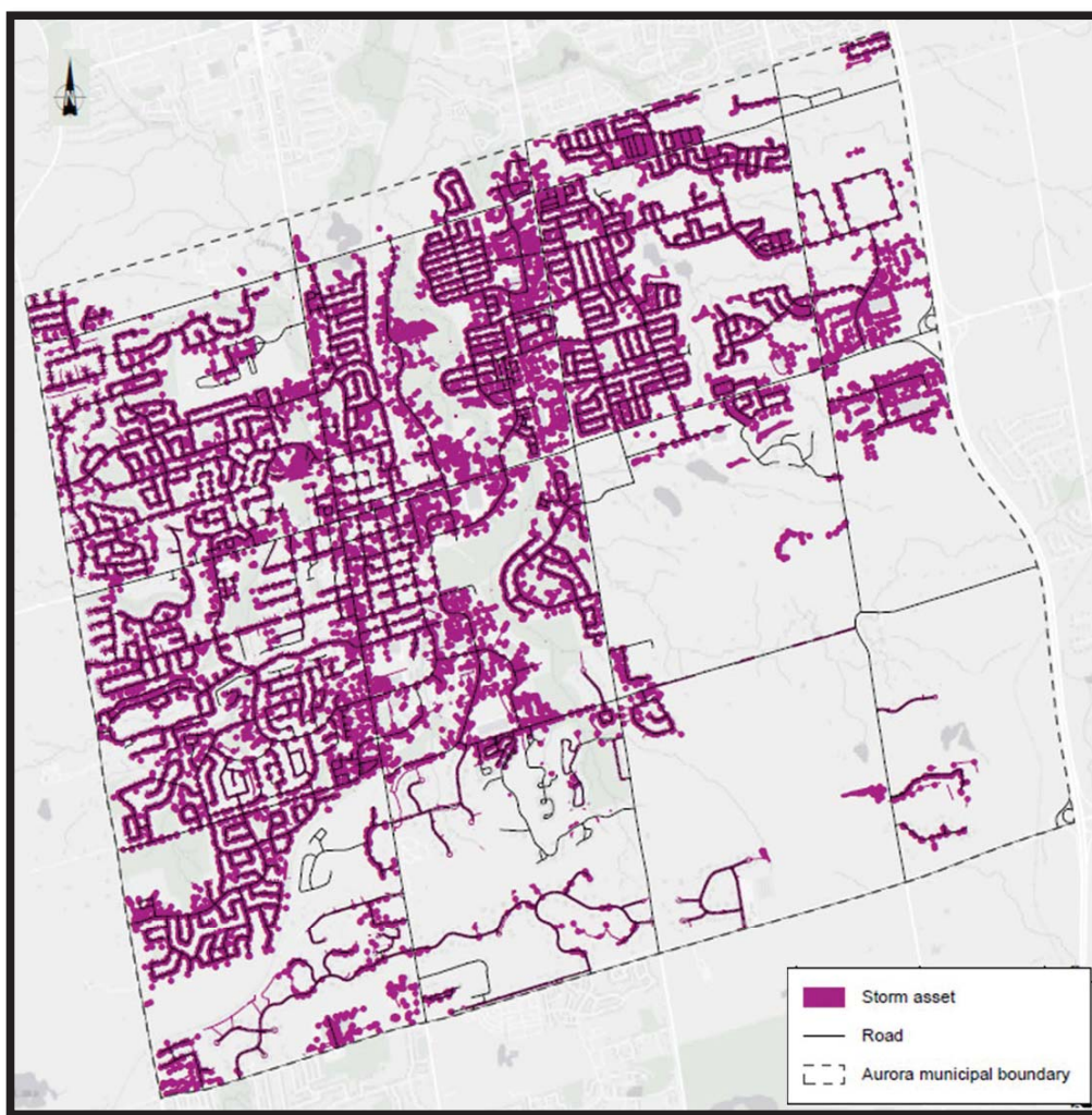
Figure 2: Map of Roads and the Stormwater Network
